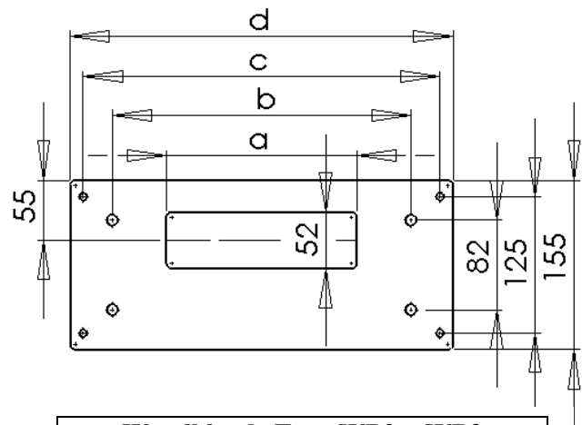
Wandblende Type WB2 + WB3
